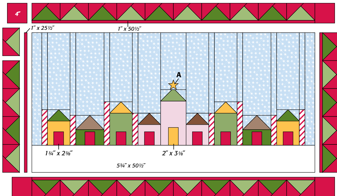
Assembly Diagram
