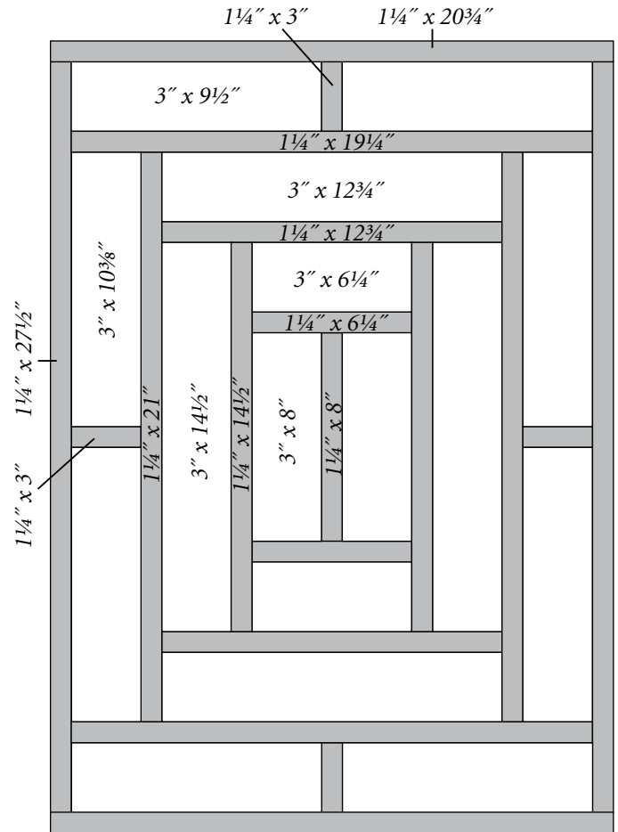
All dimensions are cutting size.
