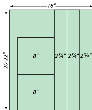
Cutting Diagram
