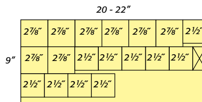
Cutting Diagram
